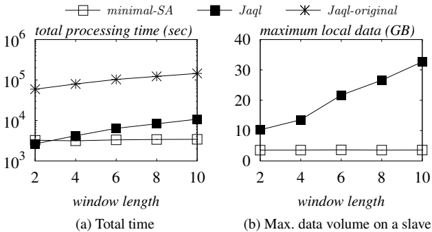
Figure 11: Sliding aggregation on small window sizes
